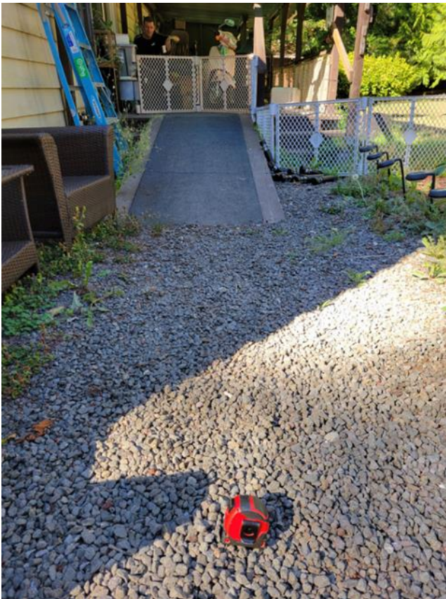
Original Ramp – tape (red) measure shows where a proper 1:12 slope ramp would end.
